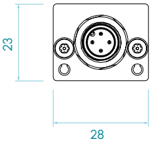
Motion sensor + M12A axial input
