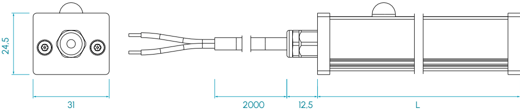
Switch + M12A radial input
