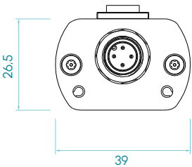
Switch + M12A radial input
