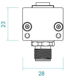
Switch + M12A radial input
